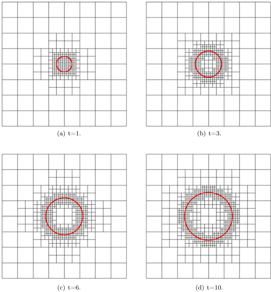
Fig. 22 Evolution of the interface and corresponding adaptive grid for Example 8.1
