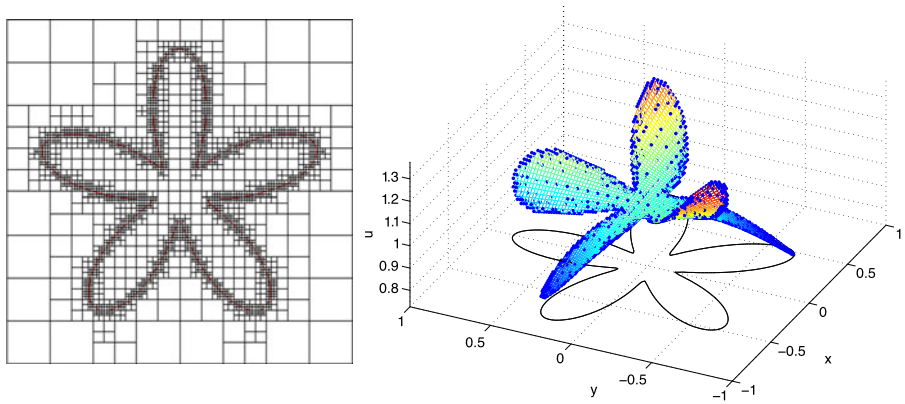
(a) Quadtree Adaptive Mesh. (b) Numerical (dots) and Exact Solutions (mesh plot).
